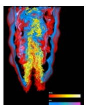
First 3-D simulation of flame that resolves chemical composition, temperature, and flow
